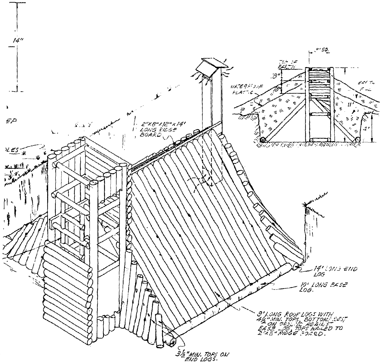
Fig. A-4.1. Two-Family A-Frame Pole Shelter, Semiburied.
